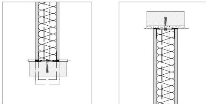
VERTICAL SECTIONS
